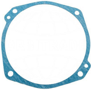
20935 Gasket between forward flange and engine, MS gear Replaces: 853935, 803227
